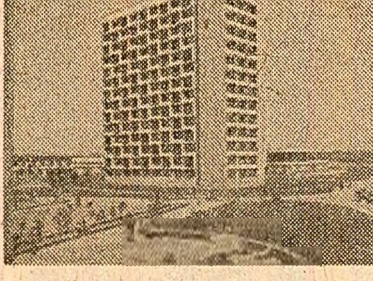
Saturn
