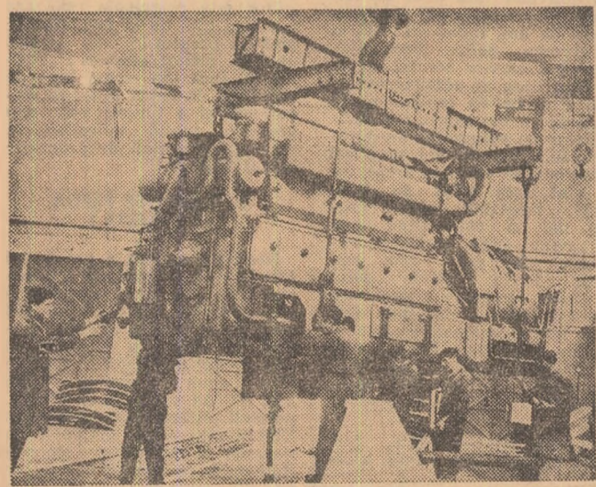
„Laboratoru” locomotivelor Diesel-electrice
